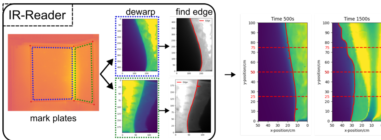
Fig. 2. Figure caption followed by period. Data-processing from the raw camera file (IBR) to CSV files to extract and analyze flame edge data. The right part indicates the locations ( y = 25 cm, 50 cm and 75 cm) of the flame spread analysis presented in this article.
