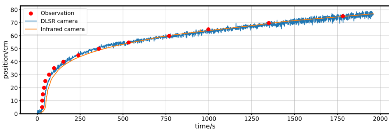
Fig. 3. Comparison between the flame front position based on optical data, IR data and data collected by an observer tracking its progress relative to predefined markers during a lateral flame spread experiment.
