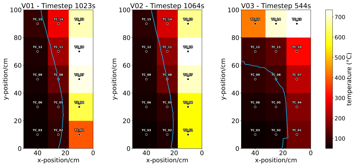
Fig. 5. Thermocouple positions and readings at the left PMMA panel, where the position indicates the distance to the center line of the experiment. The blue line shows the position of the flame front. The time steps were chosen to match the time, when the flame front reaches TC_08.
