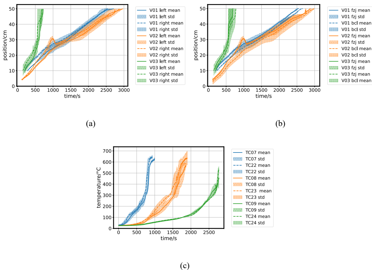
Fig. 8. Symmetry analysis based on temperature and IR measurements, all at a height of 50 cm.
