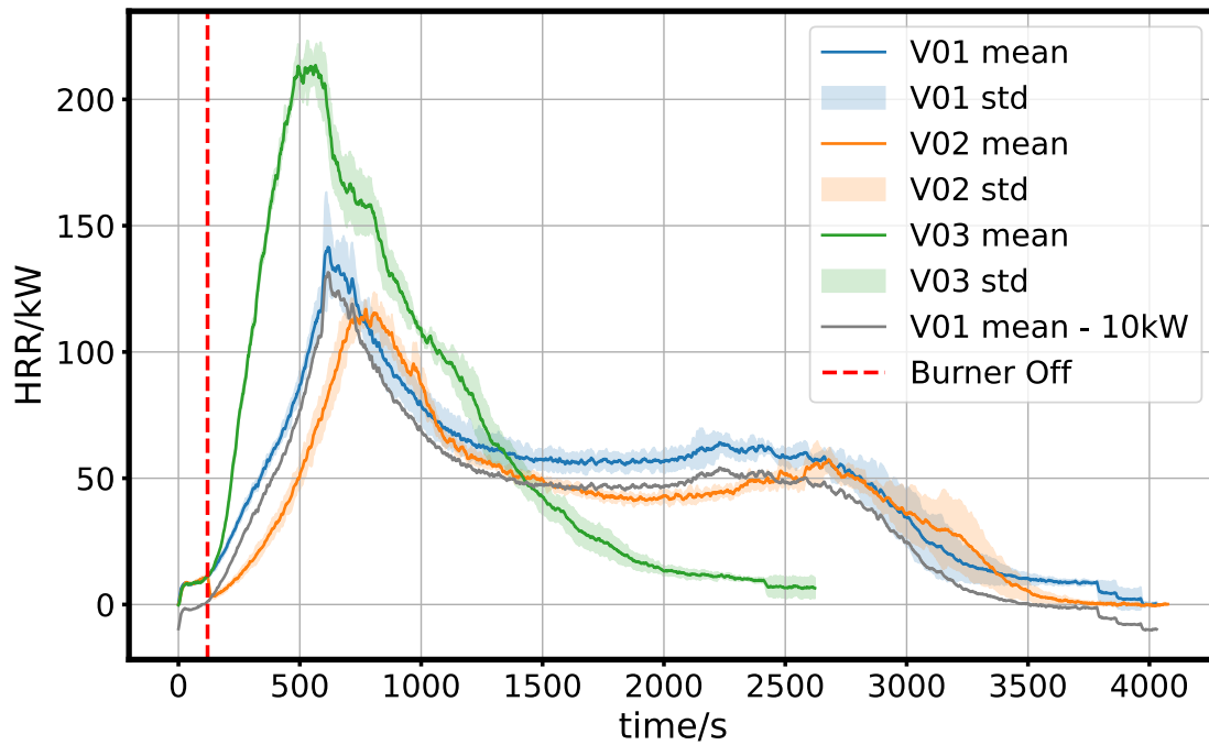
Fig. 4. Mean and standard deviation (std) of the HRR for the three different configurations. Additionally, for V01, the mean without the burner contribution (10 kW) is shown.
