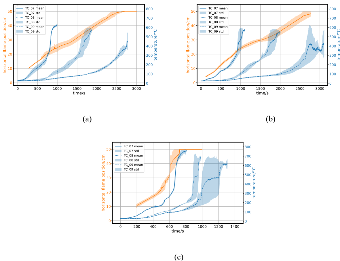
Fig. 7. Flame position at 50 cm height and temperature evolution (TC_07, TC_08, TC_09) on the left PMMA slab.
